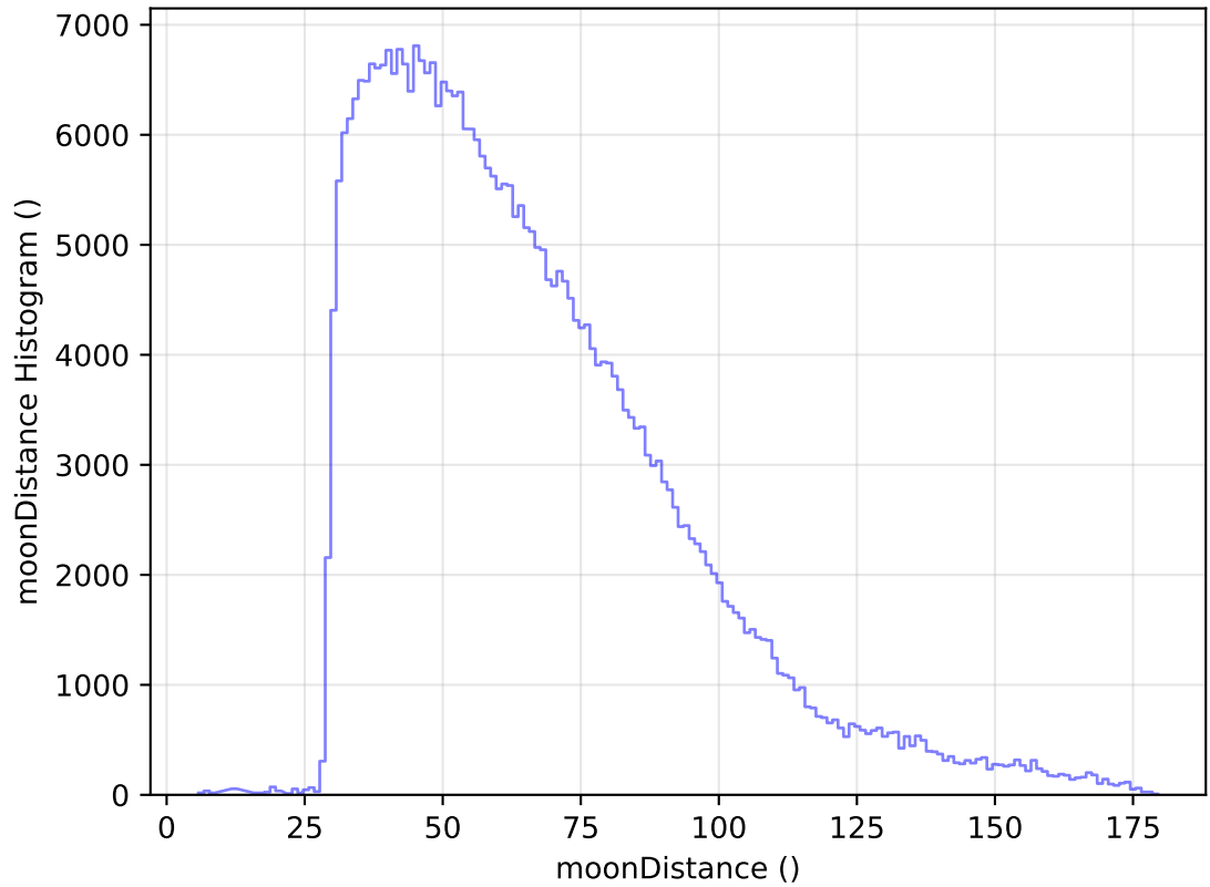
too_elab_heavy_r32_d3_griz_v3.4_10yrs WFD y band: moonDistance Histogram
