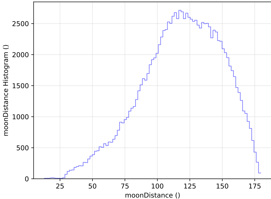
too_elab_heavy_r32_d3_griz_v3.4_10yrs WFD u band: moonDistance Histogram
