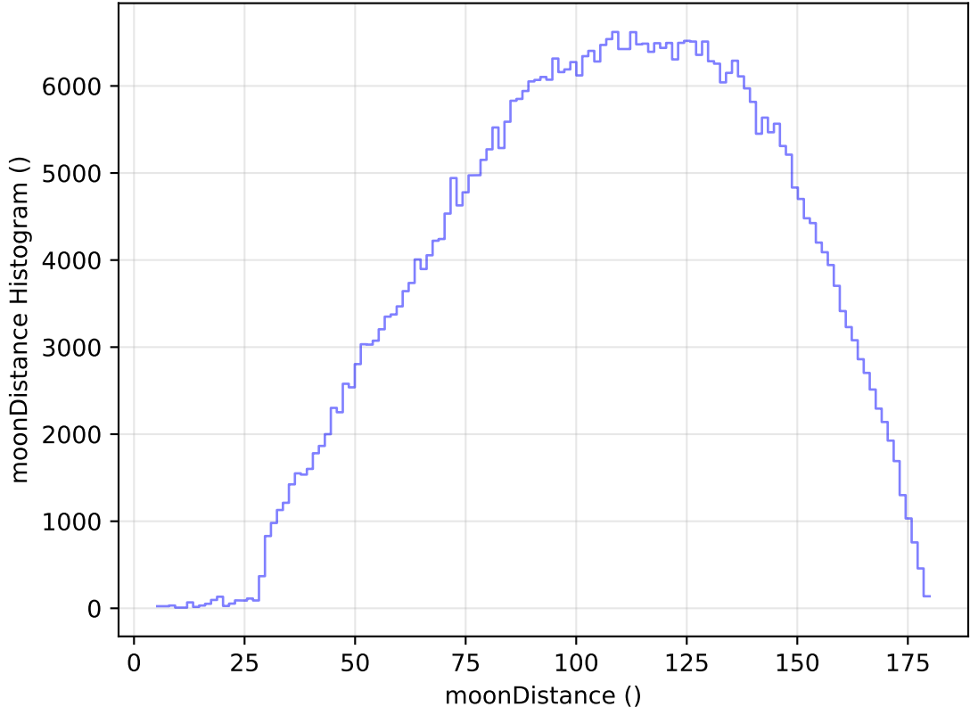
too_elab_heavy_r32_d3_griz_v3.4_10yrs WFD r band: moonDistance Histogram
