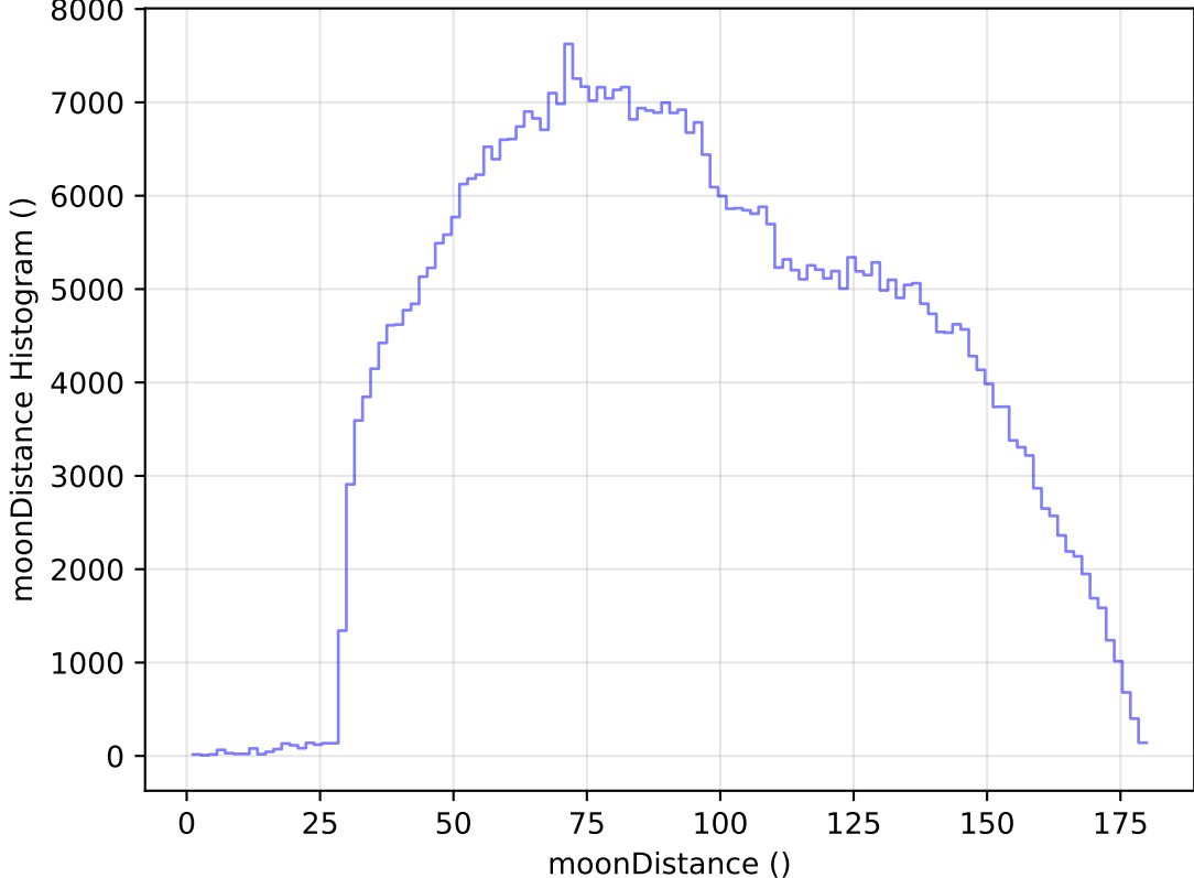
too_elab_heavy_r32_d3_griz_v3.4_10yrs WFD i band: moonDistance Histogram
