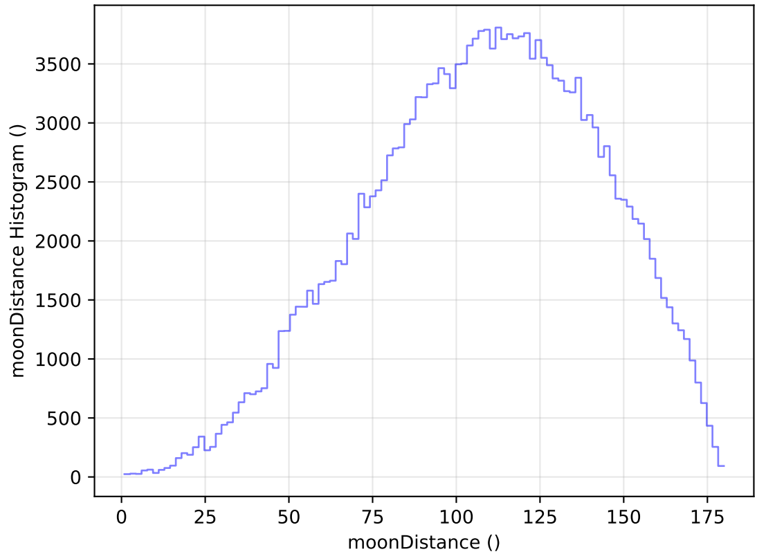
too_elab_heavy_r32_d3_griz_v3.4_10yrs WFD g band: moonDistance Histogram
