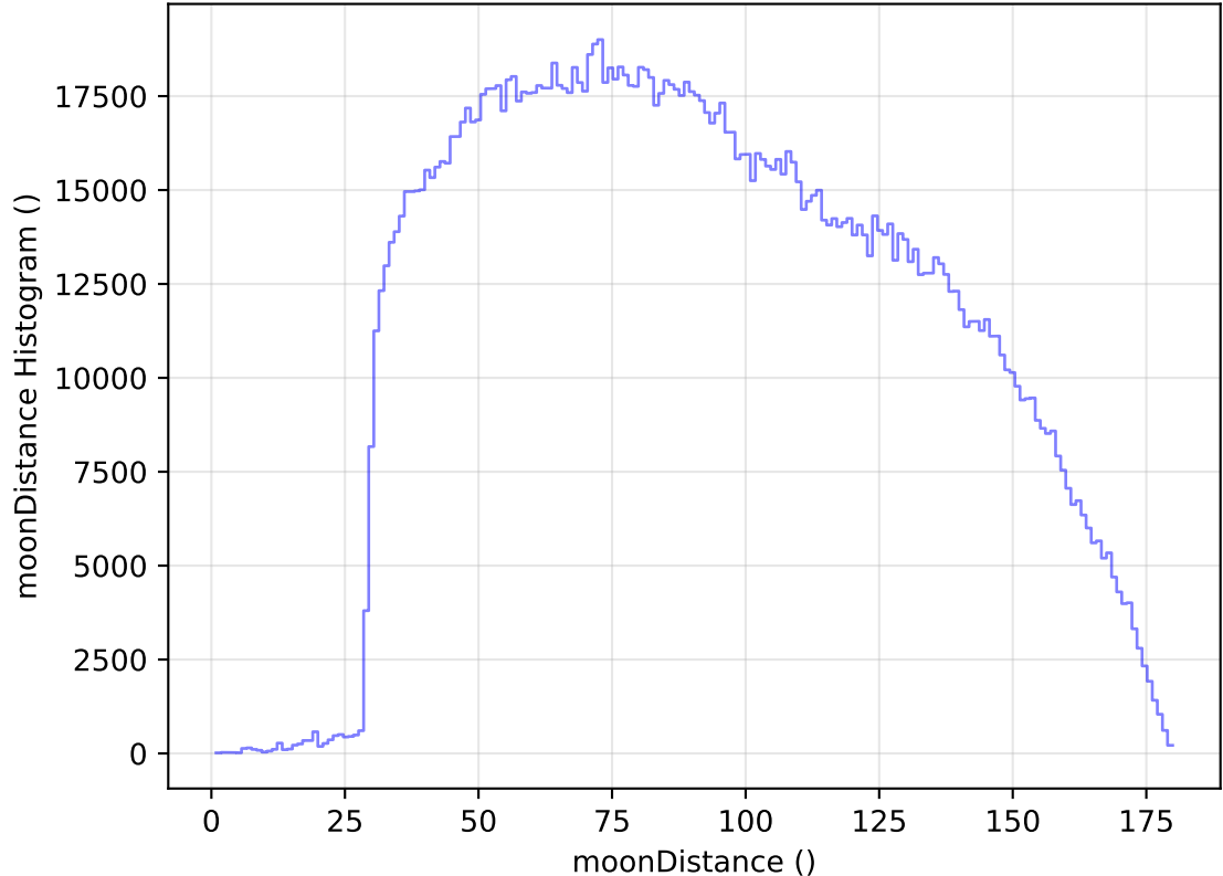
too_elab_heavy_r32_d3_griz_v3.4_10yrs WFD all bands: moonDistance Histogram
