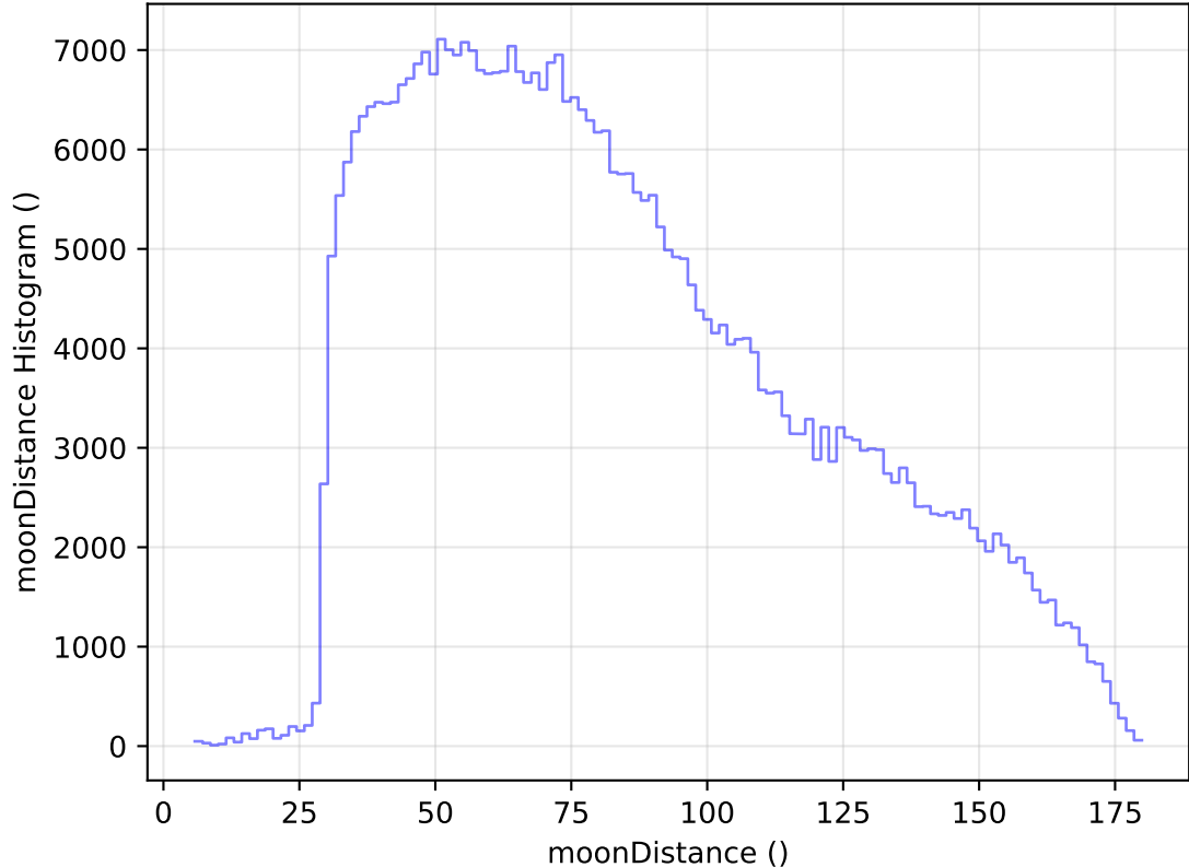
too_elab_heavy_r32_d3_griz_v3.4_10yrs All sky z band: moonDistance Histogram
