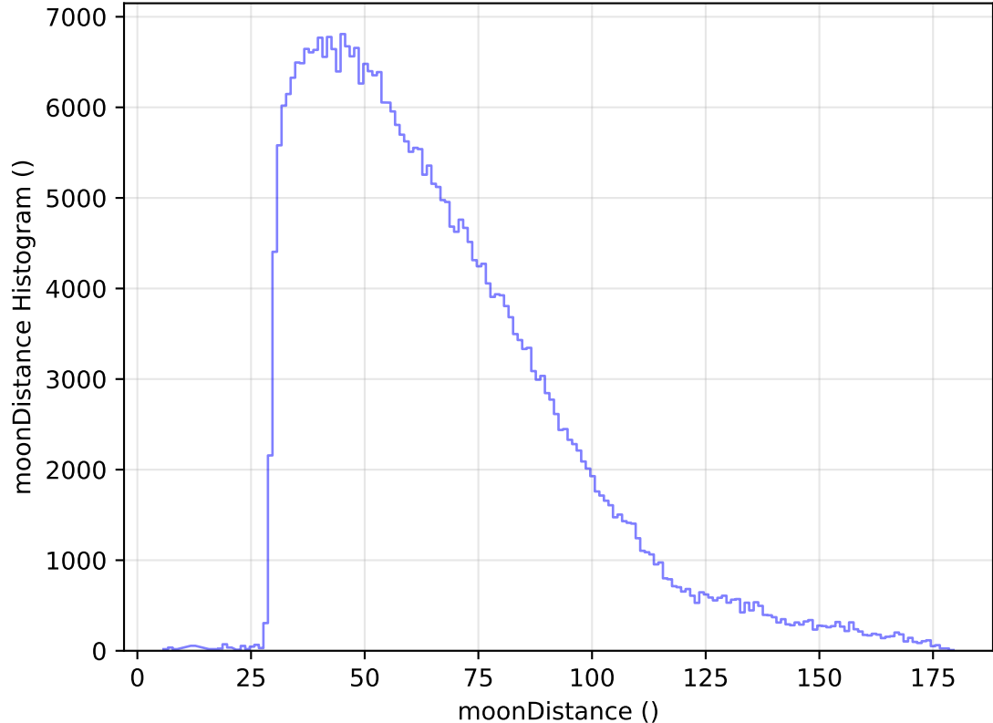
too_elab_heavy_r32_d3_griz_v3.4_10yrs All sky y band: moonDistance Histogram
