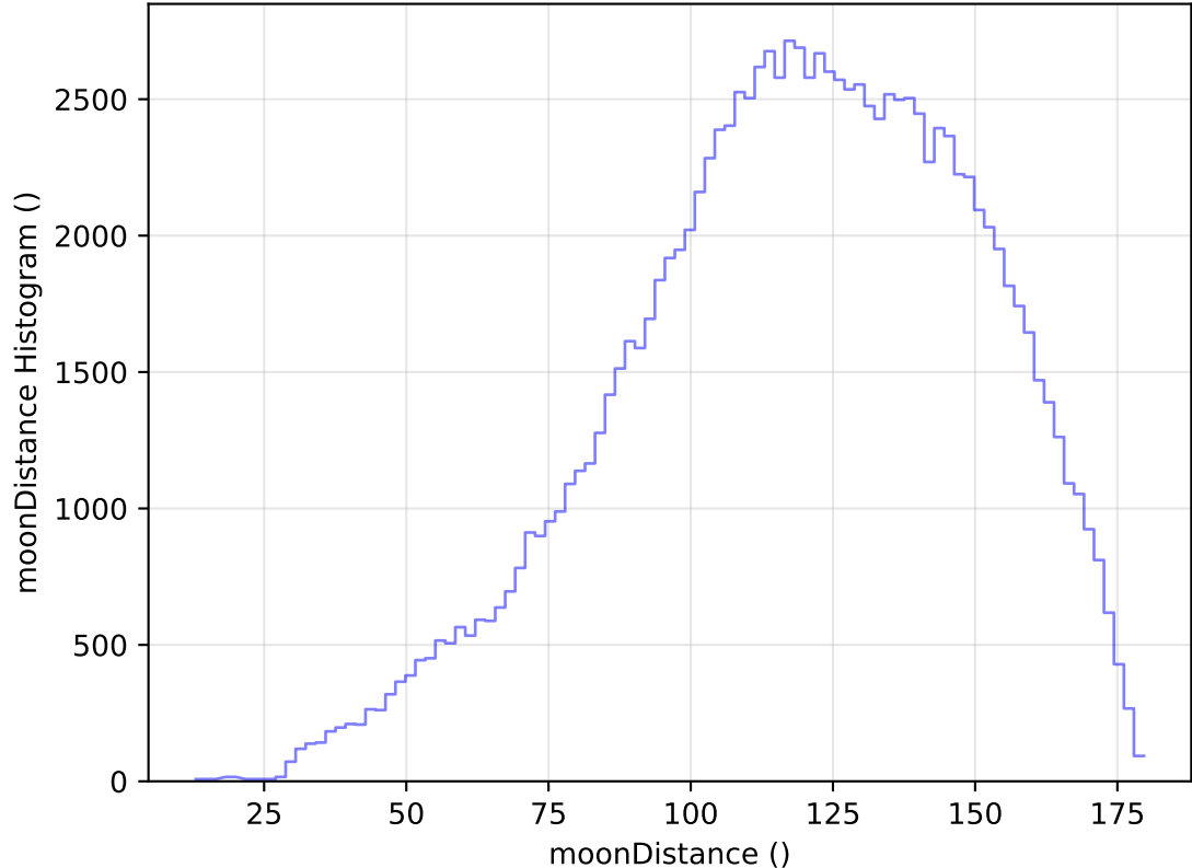
too_elab_heavy_r32_d3_griz_v3.4_10yrs All sky u band: moonDistance Histogram
