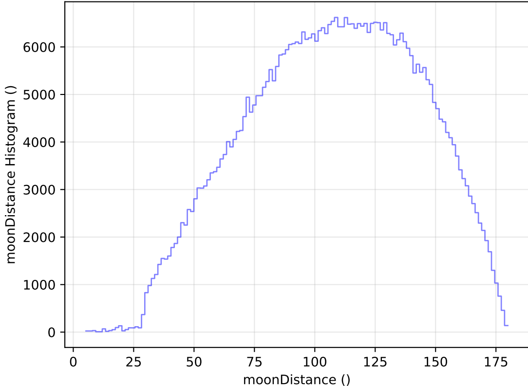
too_elab_heavy_r32_d3_griz_v3.4_10yrs All sky r band: moonDistance Histogram
