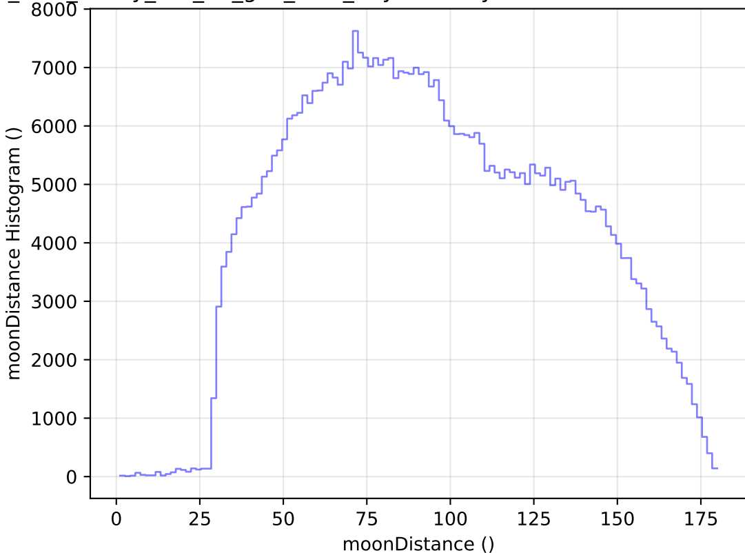
too_elab_heavy_r32_d3_griz_v3.4_10yrs All sky i band: moonDistance Histogram
