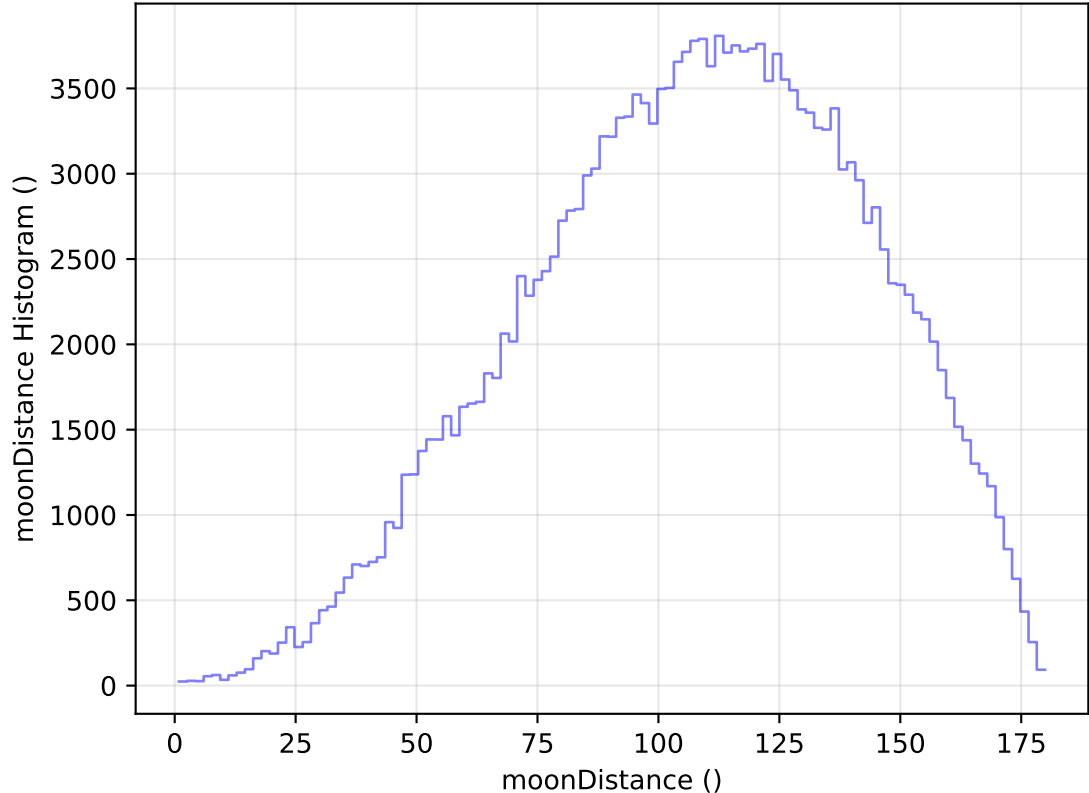
too_elab_heavy_r32_d3_griz_v3.4_10yrs All sky g band: moonDistance Histogram
