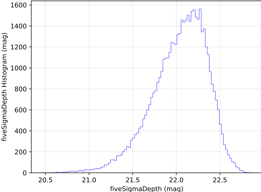
too_elab_heavy_r32_d3_griz_v3.4_10yrs Yr 1 y band: fiveSigmaDepth Histogram
