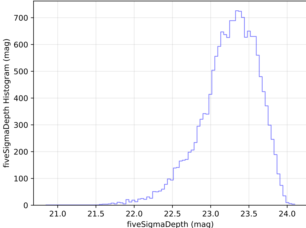
too_elab_heavy_r32_d3_griz_v3.4_10yrs Yr 1 u band: fiveSigmaDepth Histogram
