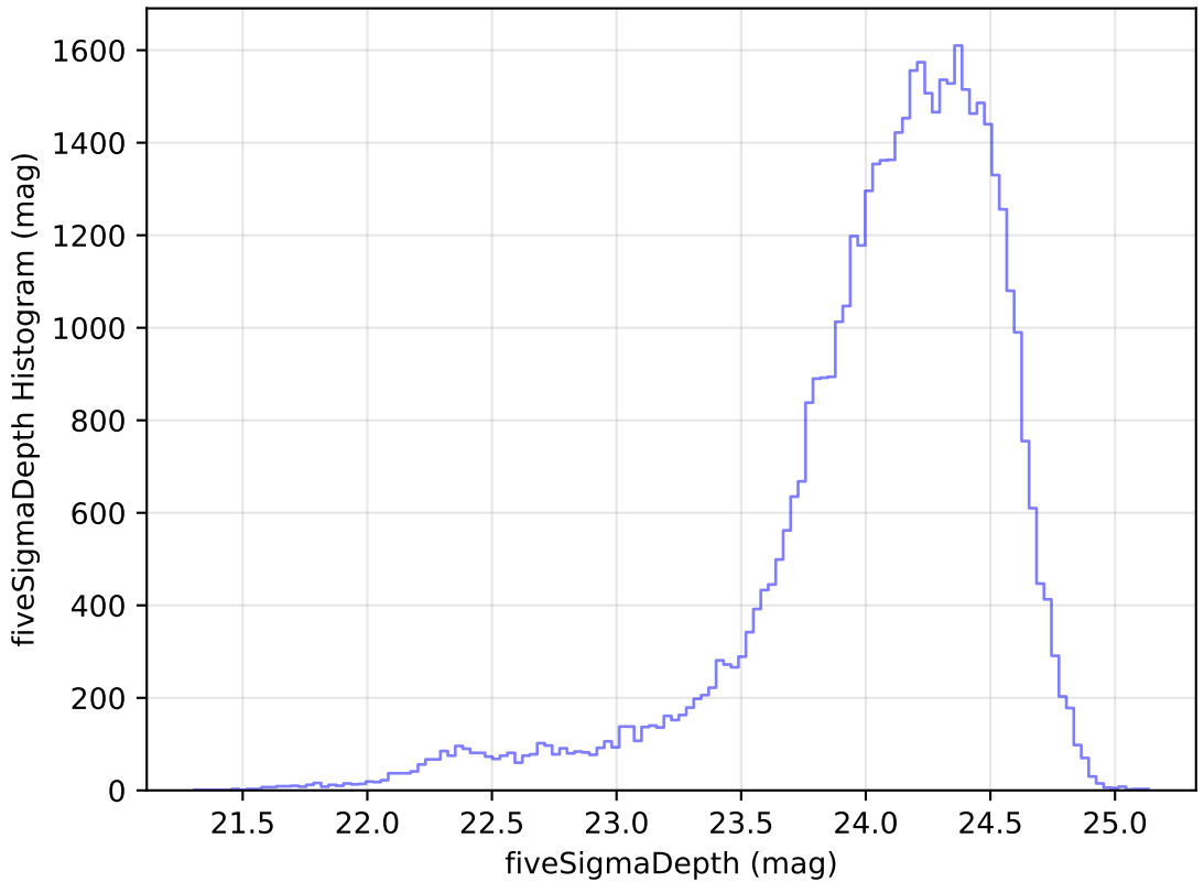
too_elab_heavy_r32_d3_griz_v3.4_10yrs Yr 1 r band: fiveSigmaDepth Histogram
