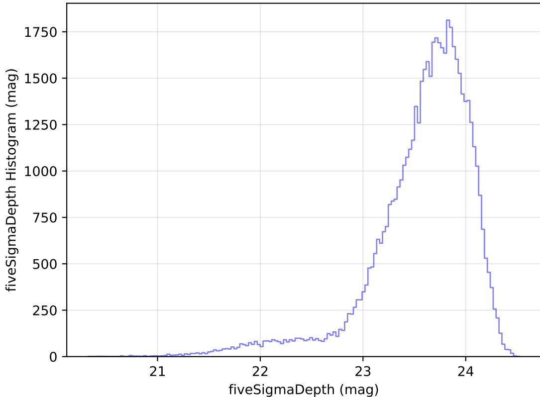
too_elab_heavy_r32_d3_griz_v3.4_10yrs Yr 1 i band: fiveSigmaDepth Histogram
