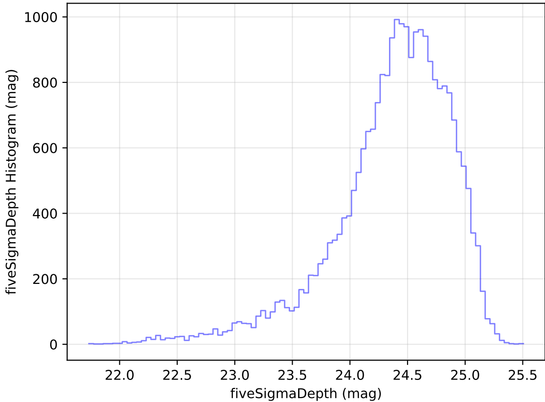
too_elab_heavy_r32_d3_griz_v3.4_10yrs Yr 1 g band: fiveSigmaDepth Histogram
