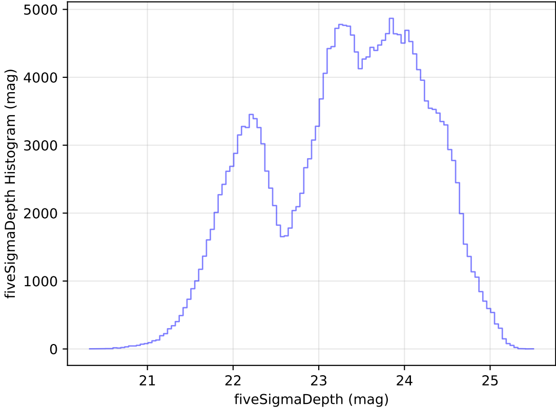
too_elab_heavy_r32_d3_griz_v3.4_10yrs Yr 1 all bands: fiveSigmaDepth Histogram
