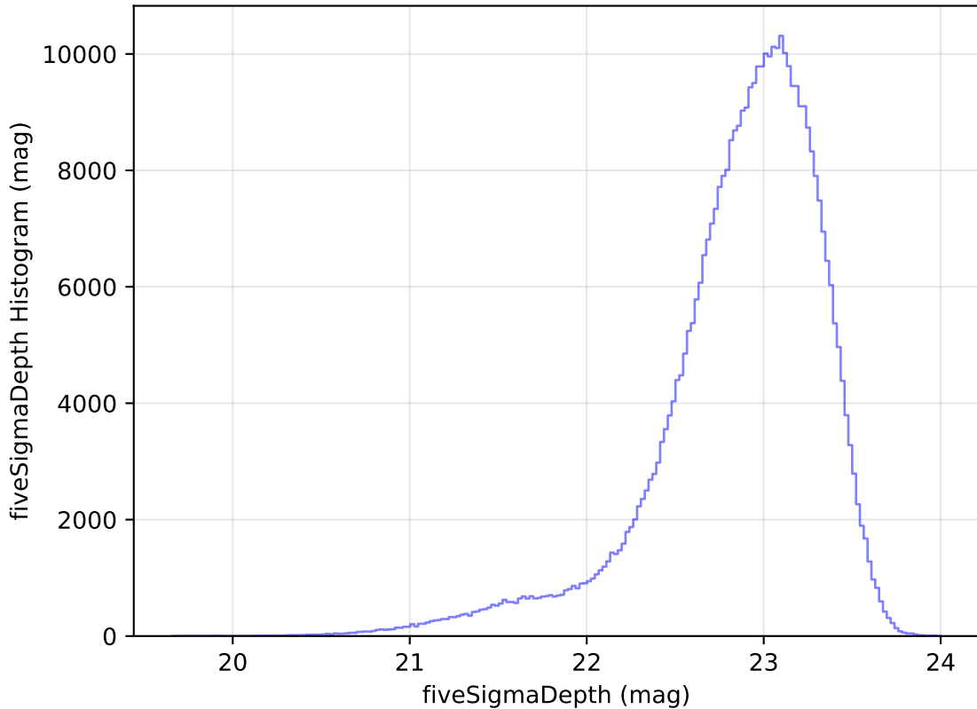
too_elab_heavy_r32_d3_griz_v3.4_10yrs WFD z band: fiveSigmaDepth Histogram
