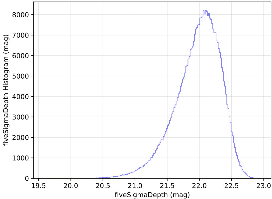
too_elab_heavy_r32_d3_griz_v3.4_10yrs WFD y band: fiveSigmaDepth Histogram
