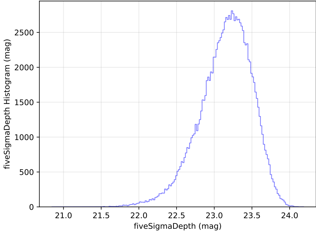
too_elab_heavy_r32_d3_griz_v3.4_10yrs WFD u band: fiveSigmaDepth Histogram
