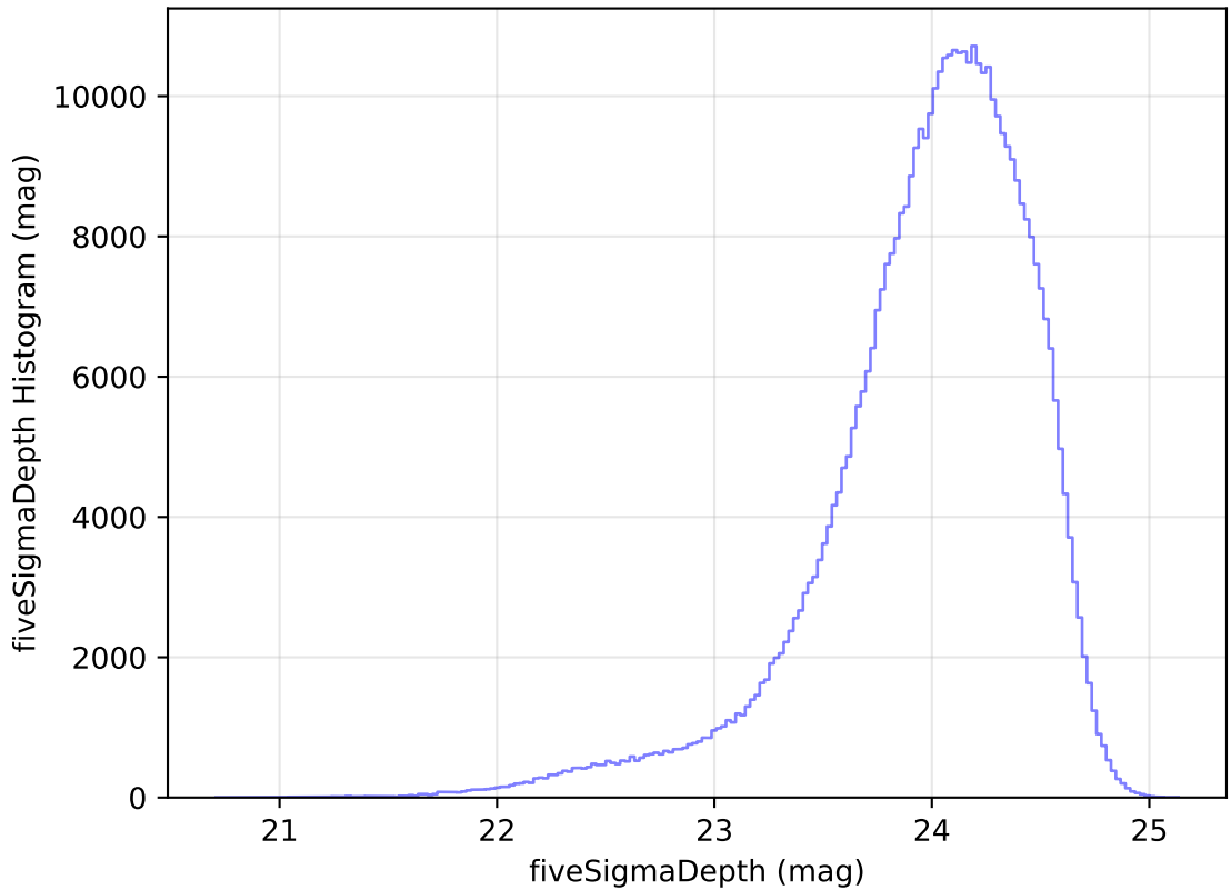
too_elab_heavy_r32_d3_griz_v3.4_10yrs WFD r band: fiveSigmaDepth Histogram
