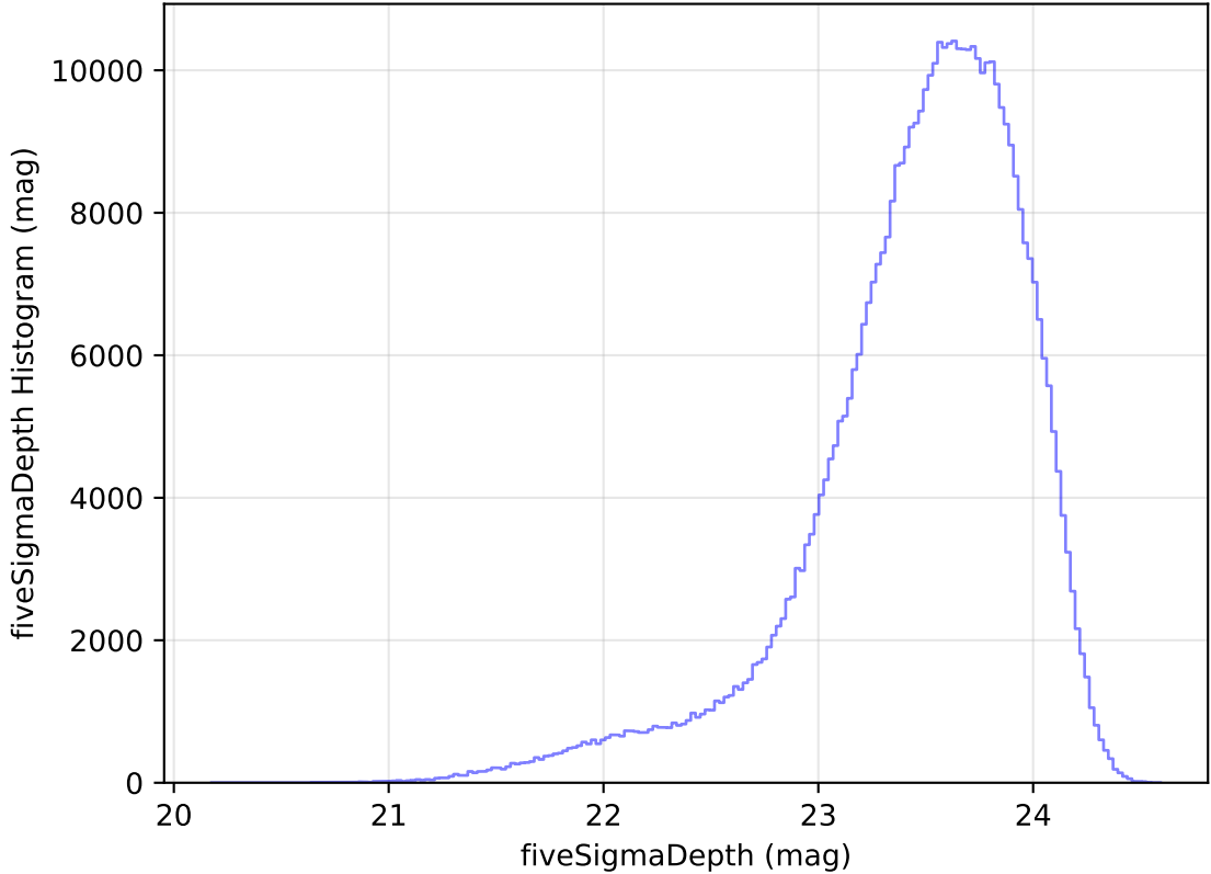
too_elab_heavy_r32_d3_griz_v3.4_10yrs WFD i band: fiveSigmaDepth Histogram
