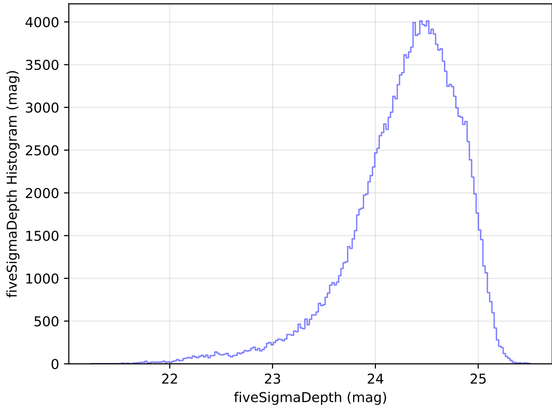
too_elab_heavy_r32_d3_griz_v3.4_10yrs WFD g band: fiveSigmaDepth Histogram
