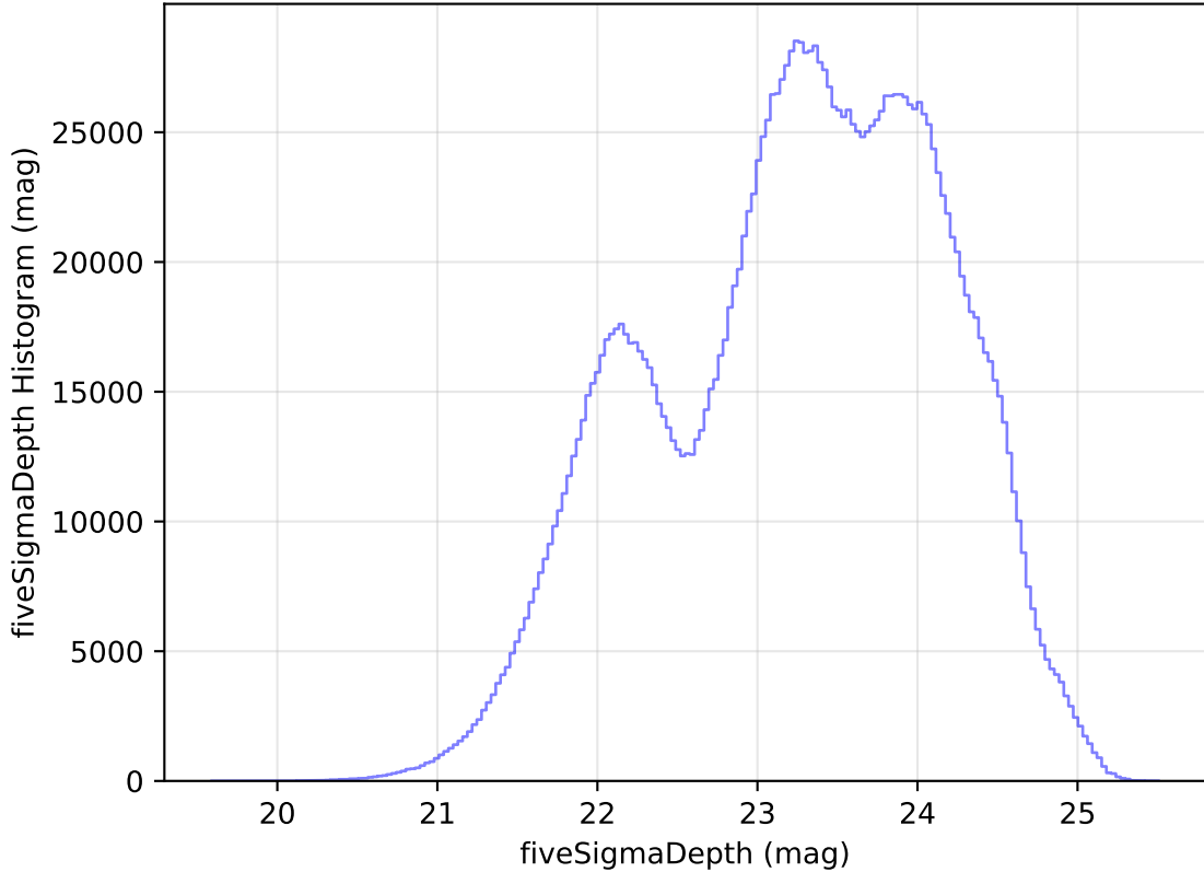
too_elab_heavy_r32_d3_griz_v3.4_10yrs WFD all bands: fiveSigmaDepth Histogram
