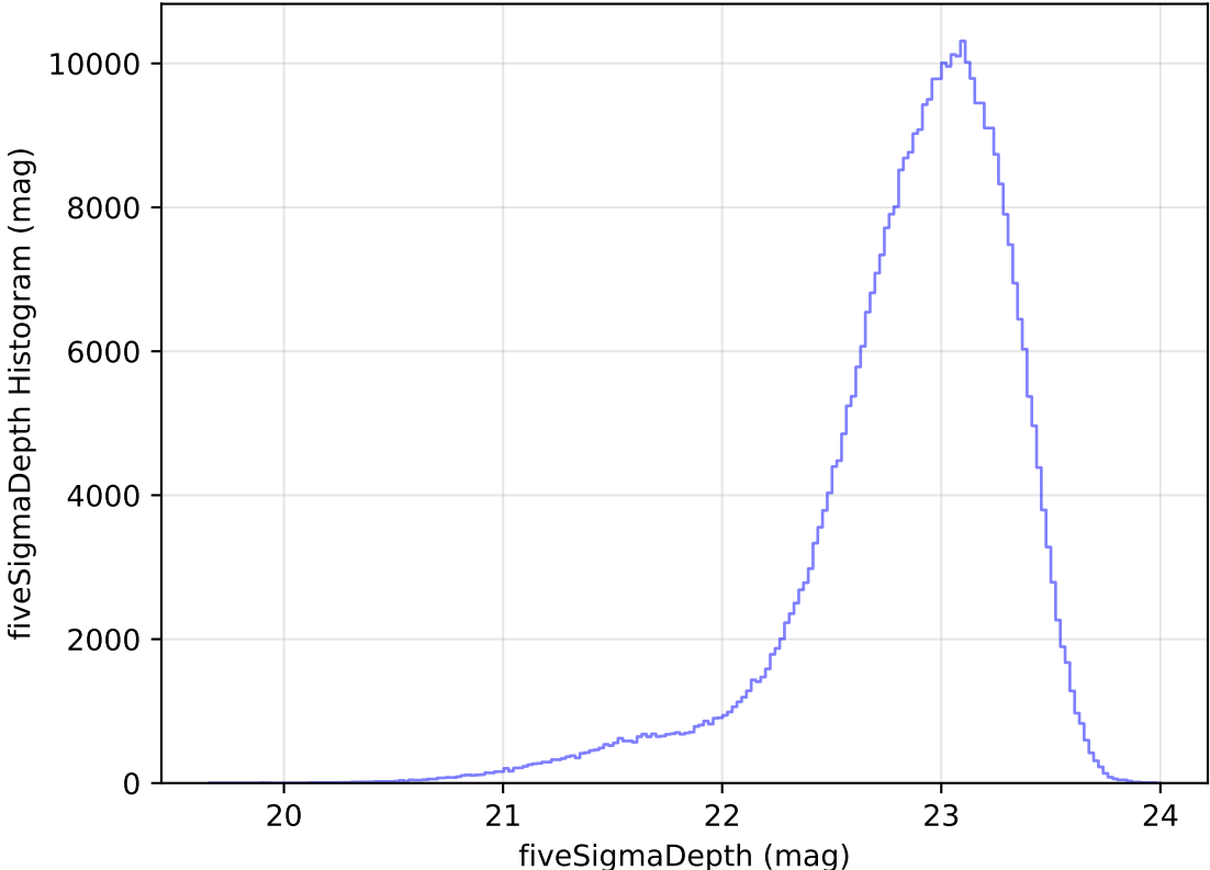
too_elab_heavy_r32_d3_griz_v3.4_10yrs All sky z band: fiveSigmaDepth Histogram
