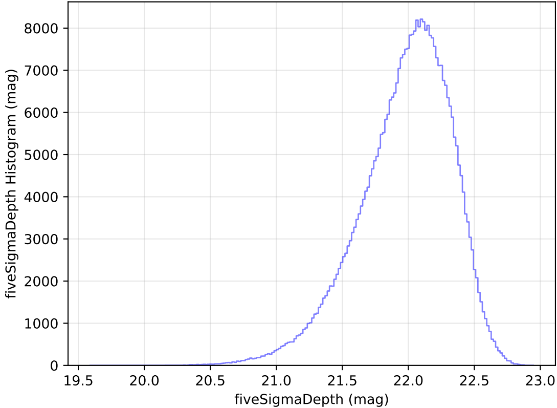
too_elab_heavy_r32_d3_griz_v3.4_10yrs All sky y band: fiveSigmaDepth Histogram
