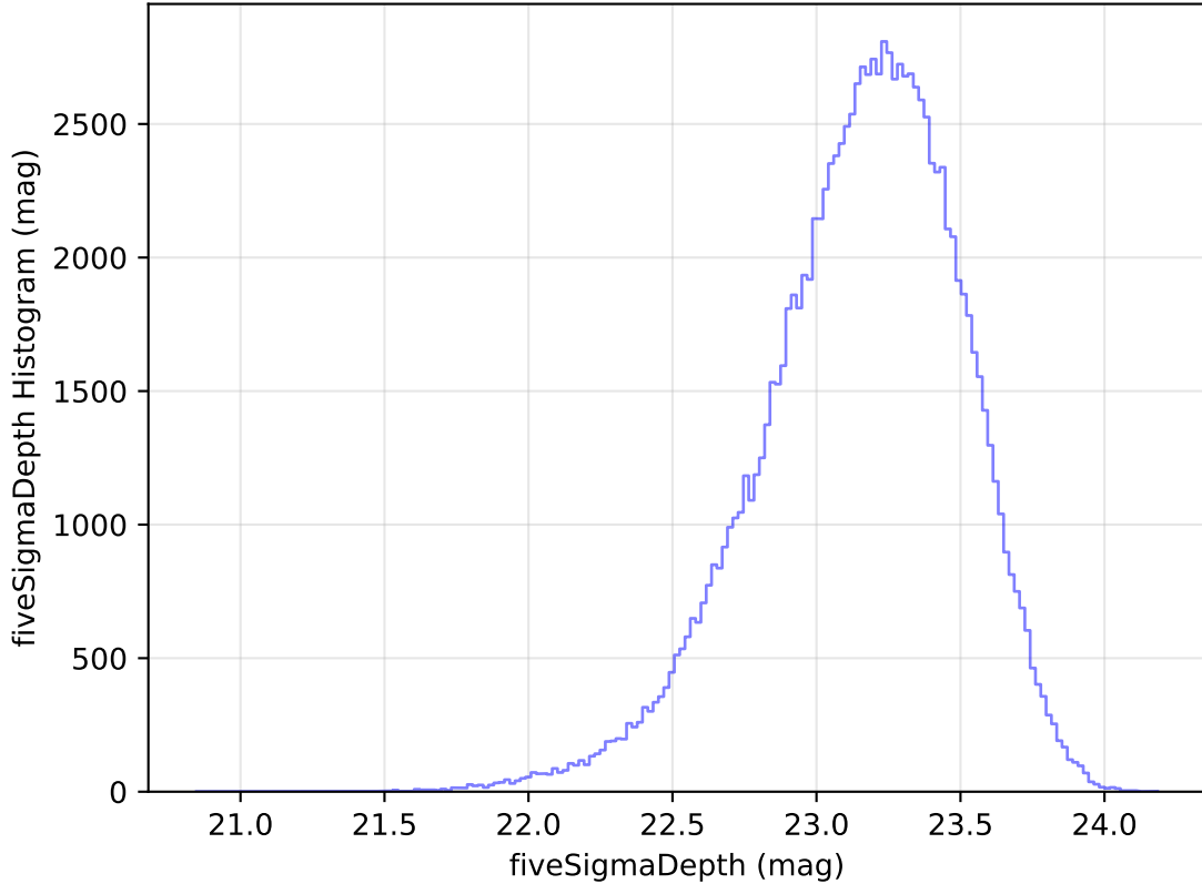
too_elab_heavy_r32_d3_griz_v3.4_10yrs All sky u band: fiveSigmaDepth Histogram
