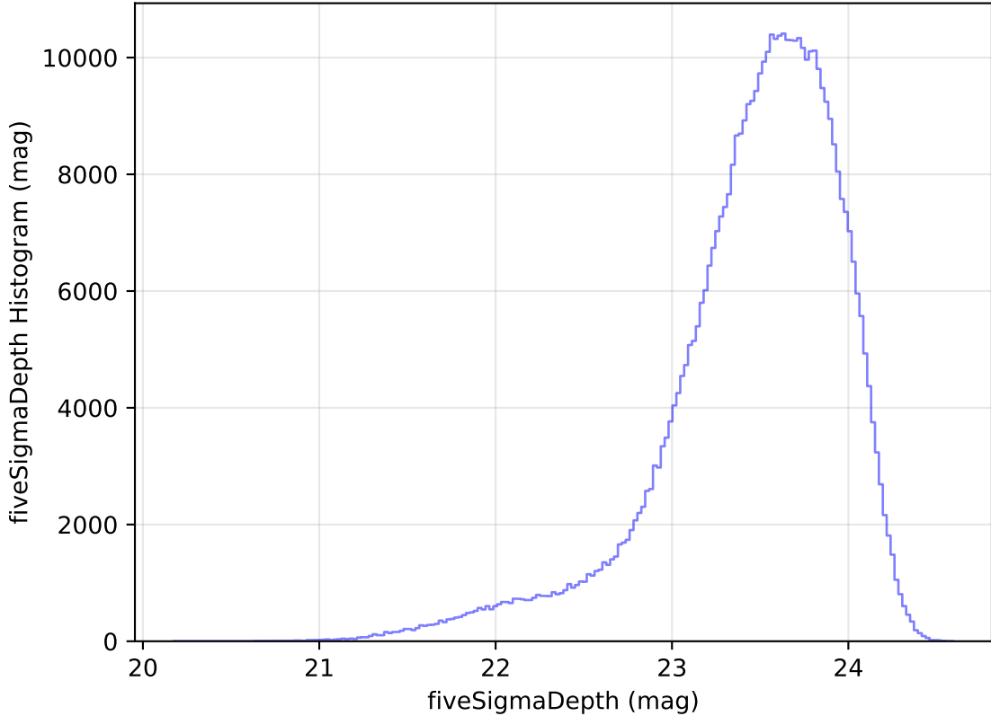
too_elab_heavy_r32_d3_griz_v3.4_10yrs All sky i band: fiveSigmaDepth Histogram
