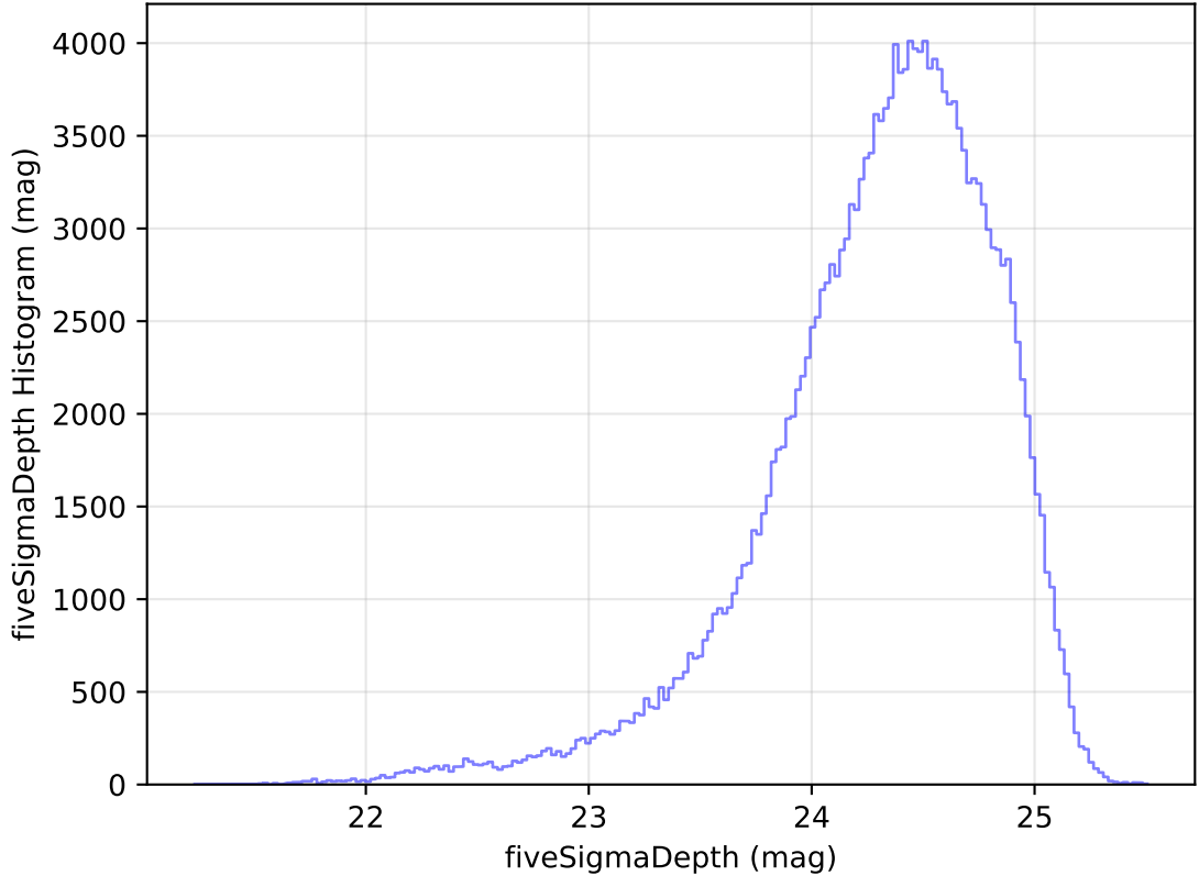
too_elab_heavy_r32_d3_griz_v3.4_10yrs All sky g band: fiveSigmaDepth Histogram
