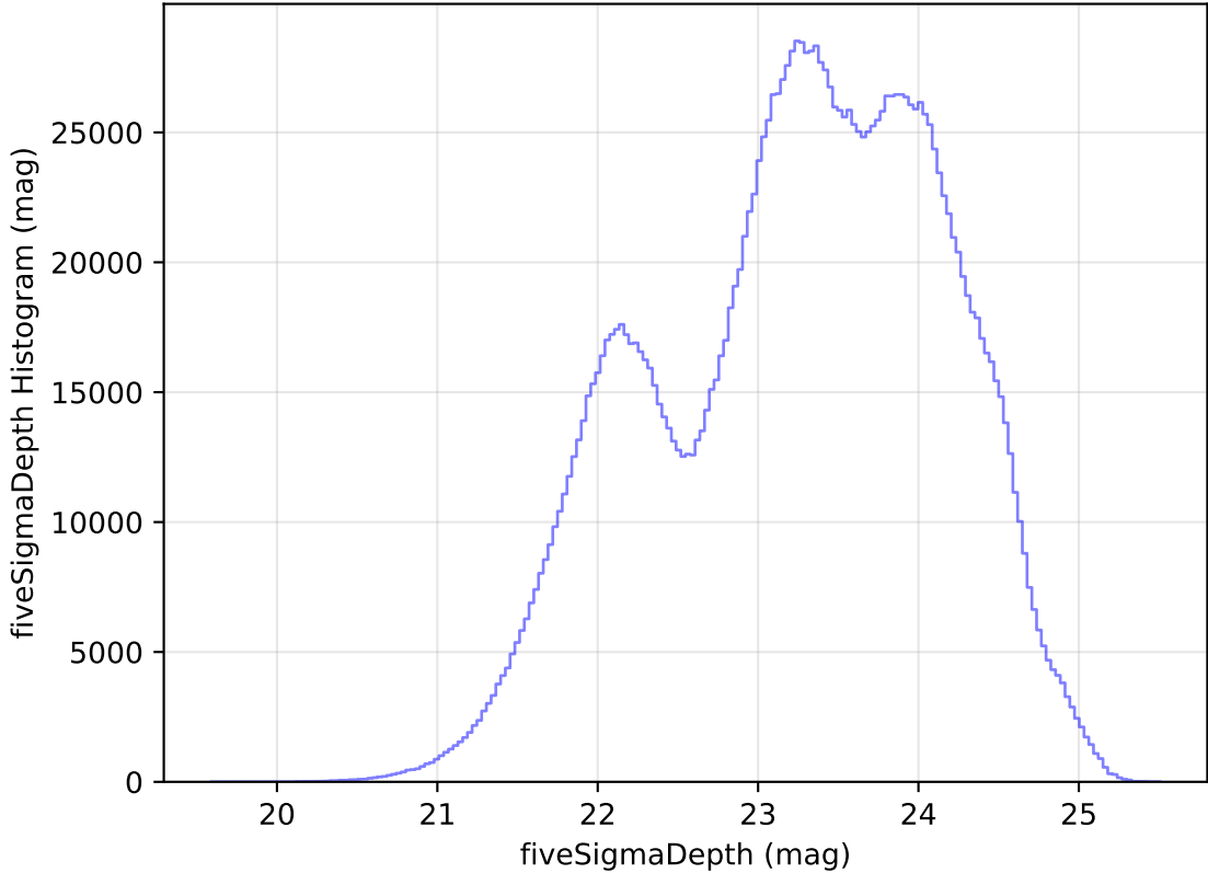
too_elab_heavy_r32_d3_griz_v3.4_10yrs All sky all bands: fiveSigmaDepth Histogram
