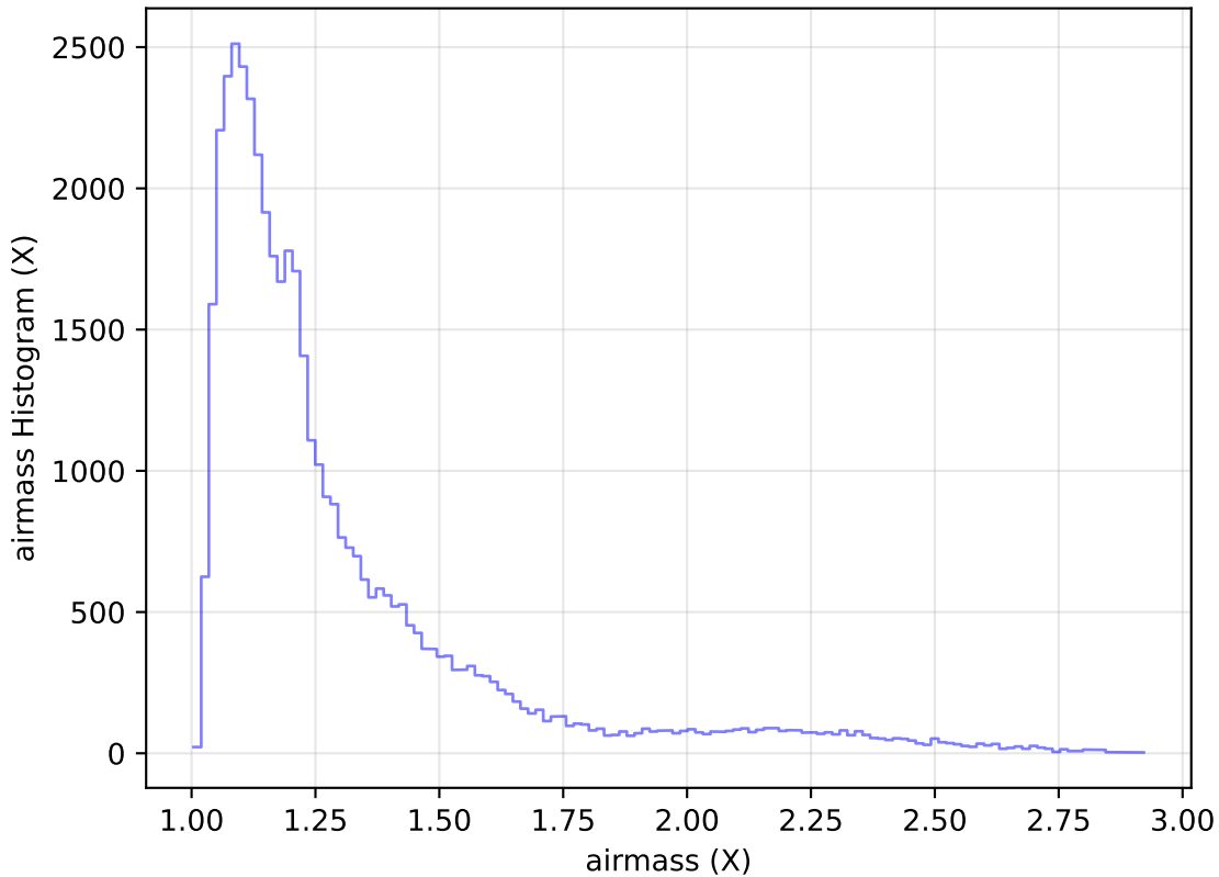
too_elab_heavy_r32_d3_griz_v3.4_10yrs Yr 1 z band: airmass Histogram
