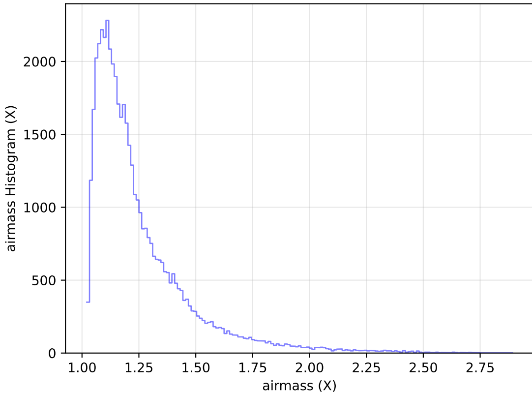
too_elab_heavy_r32_d3_griz_v3.4_10yrs Yr 1 y band: airmass Histogram
