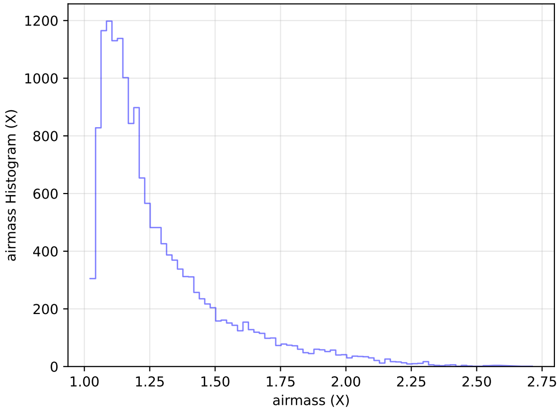
too_elab_heavy_r32_d3_griz_v3.4_10yrs Yr 1 u band: airmass Histogram
