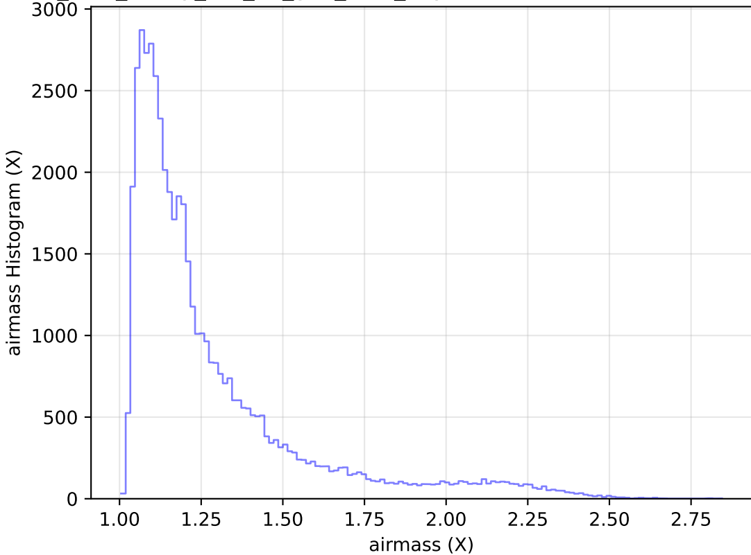
too_elab_heavy_r32_d3_griz_v3.4_10yrs Yr 1 r band: airmass Histogram
