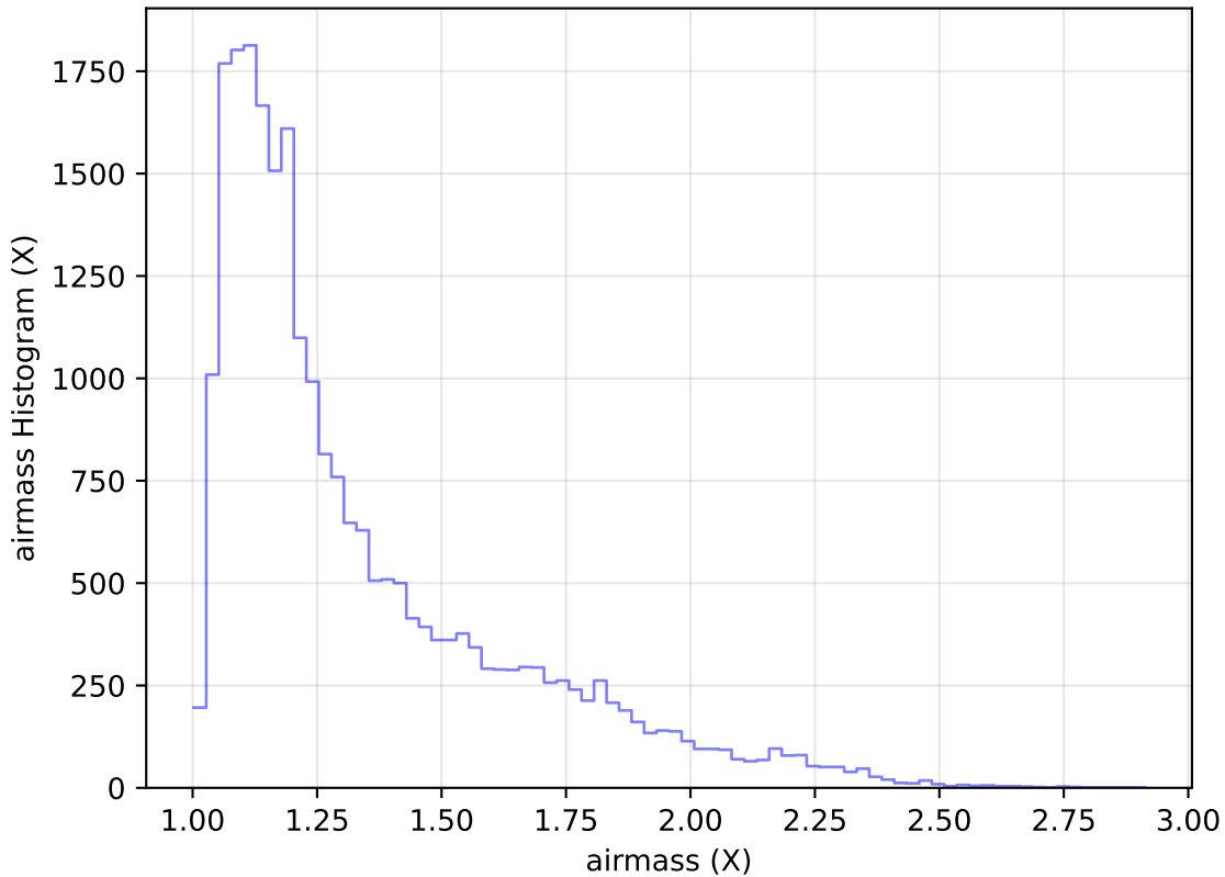
too_elab_heavy_r32_d3_griz_v3.4_10yrs Yr 1 g band: airmass Histogram
