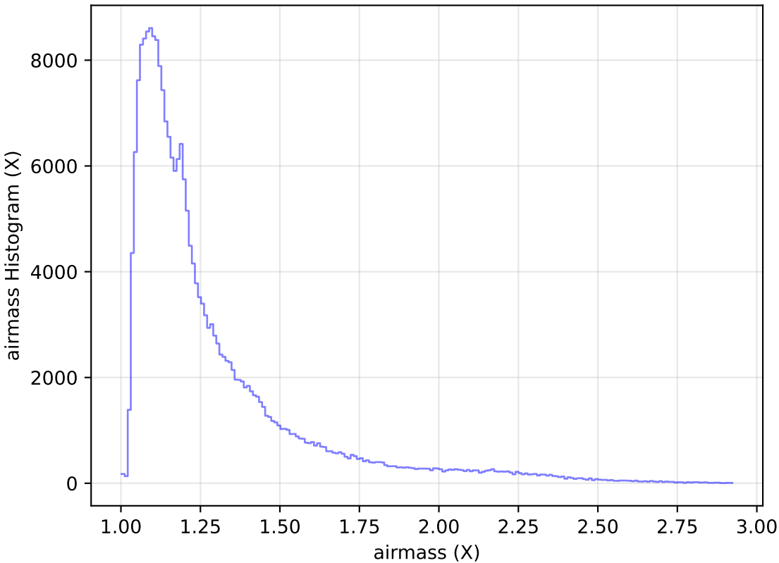
too_elab_heavy_r32_d3_griz_v3.4_10yrs Yr 1 all bands: airmass Histogram
