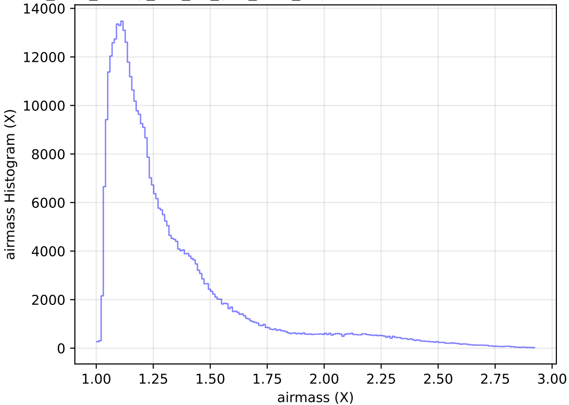
too_elab_heavy_r32_d3_griz_v3.4_10yrs WFD z band: airmass Histogram
