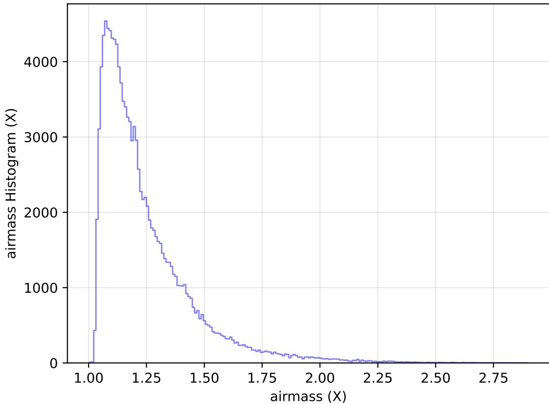
too_elab_heavy_r32_d3_griz_v3.4_10yrs WFD u band: airmass Histogram
