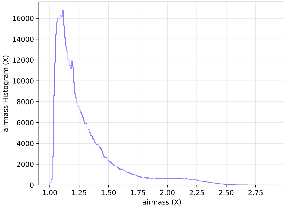
too_elab_heavy_r32_d3_griz_v3.4_10yrs WFD r band: airmass Histogram
