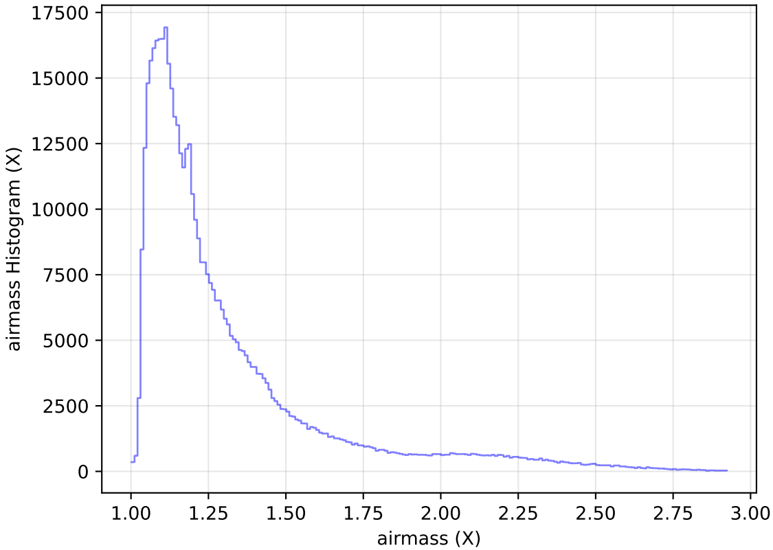
too_elab_heavy_r32_d3_griz_v3.4_10yrs WFD i band: airmass Histogram
