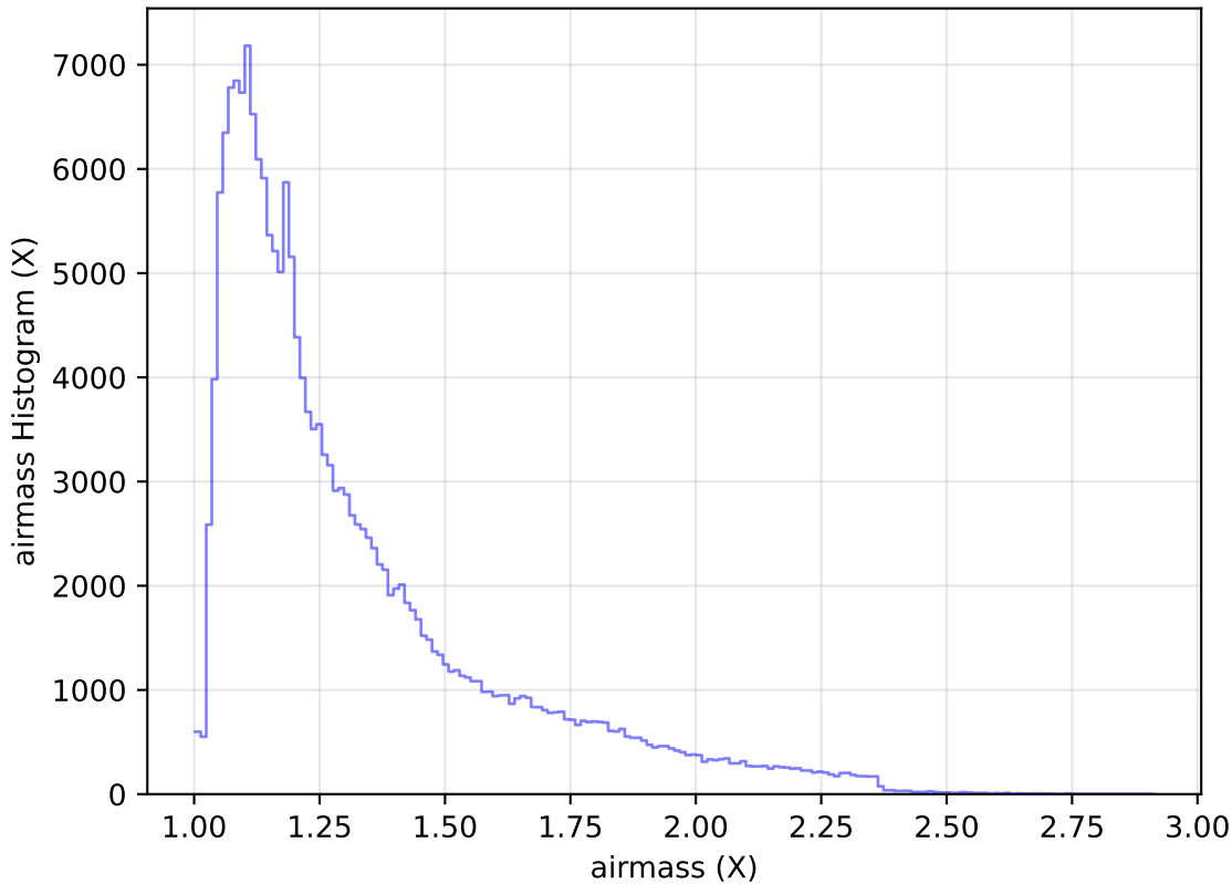
too_elab_heavy_r32_d3_griz_v3.4_10yrs WFD g band: airmass Histogram
