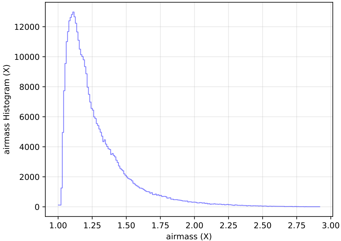
too_elab_heavy_r32_d3_griz_v3.4_10yrs All sky y band: airmass Histogram
