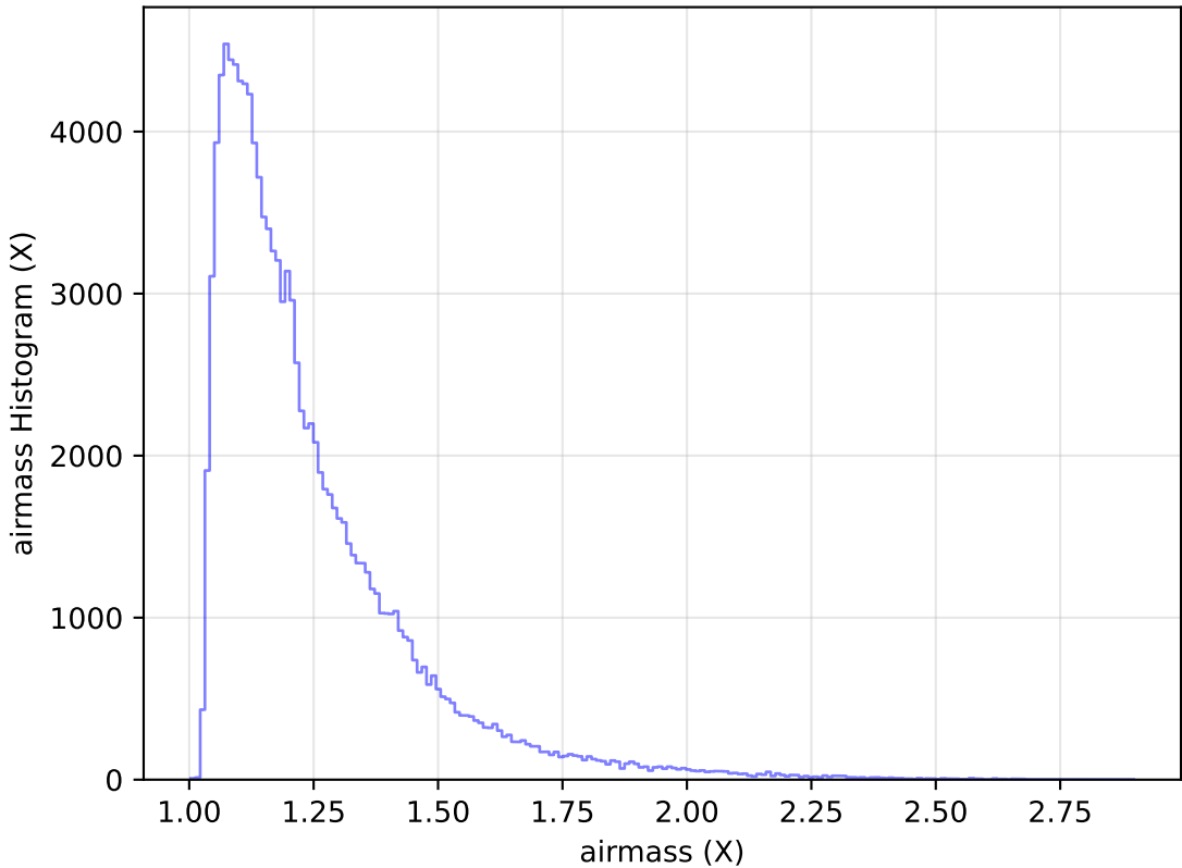
too_elab_heavy_r32_d3_griz_v3.4_10yrs All sky u band: airmass Histogram
