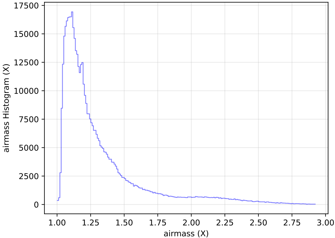
too_elab_heavy_r32_d3_griz_v3.4_10yrs All sky i band: airmass Histogram
