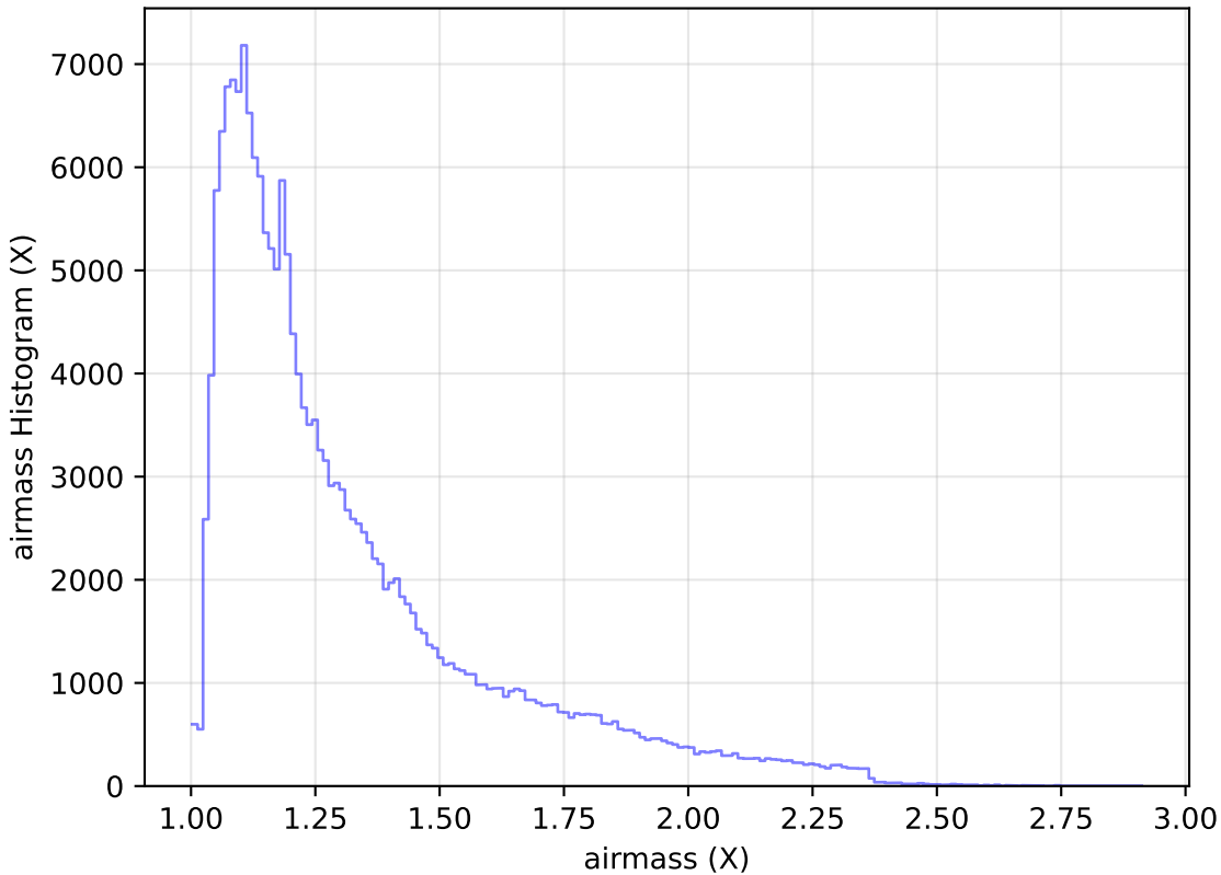
too_elab_heavy_r32_d3_griz_v3.4_10yrs All sky g band: airmass Histogram
