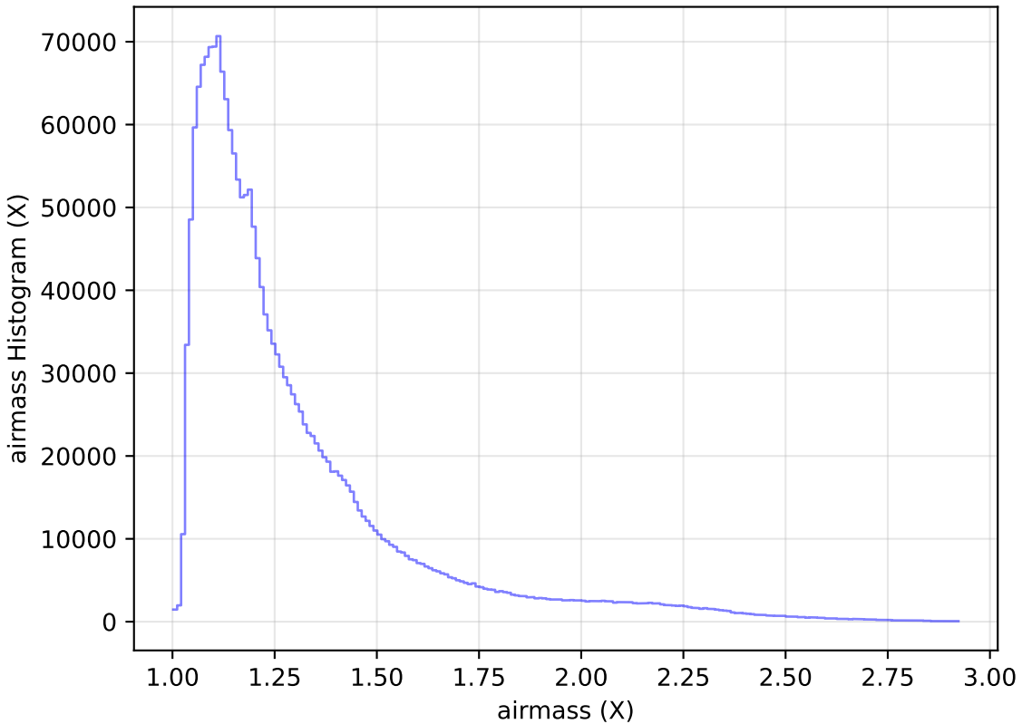
too_elab_heavy_r32_d3_griz_v3.4_10yrs All sky all bands: airmass Histogram
