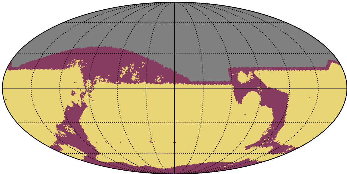
too_elab_heavy_r32_d3_griz_v3.4_10yrs All sky: RapidRevisits
