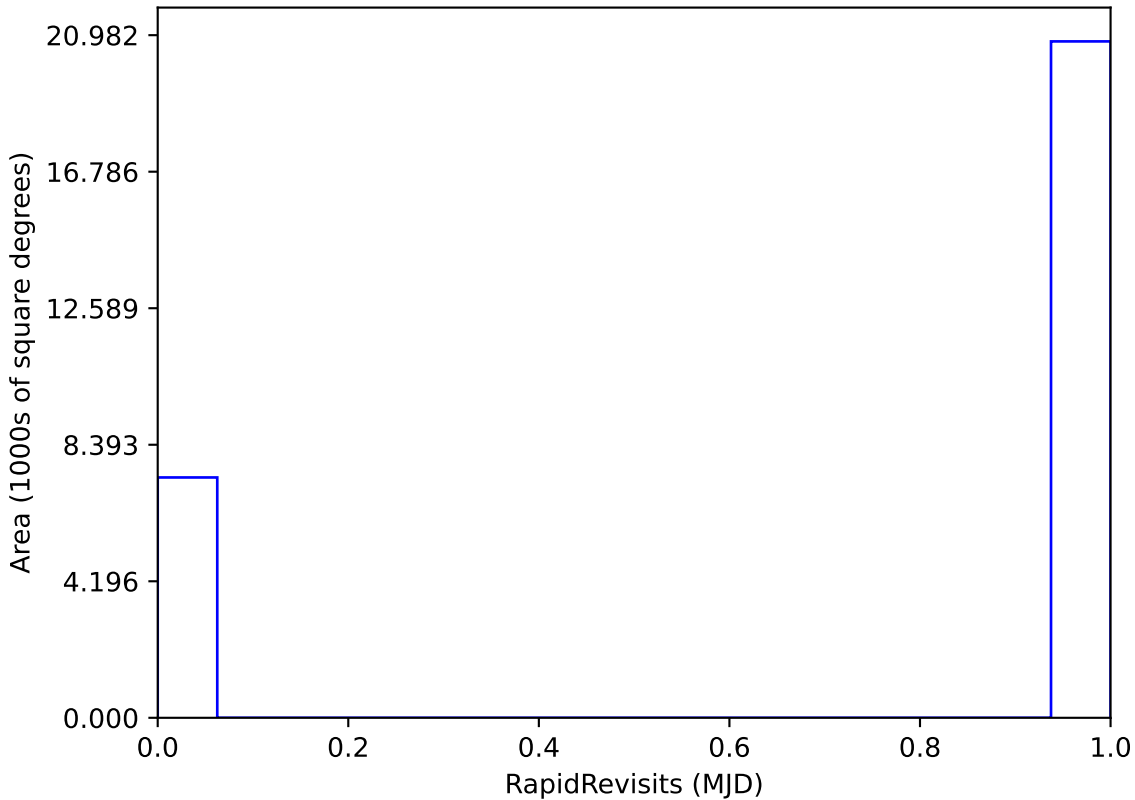
too_elab_heavy_r32_d3_griz_v3.4_10yrs All sky: RapidRevisits
