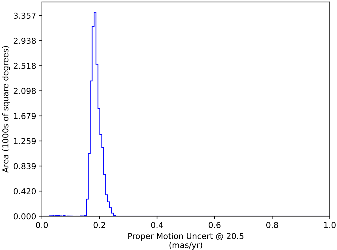
too_elab_heavy_r32_d3_griz_v3.4_10yrs WFD: Proper Motion Uncert @ 20.5
